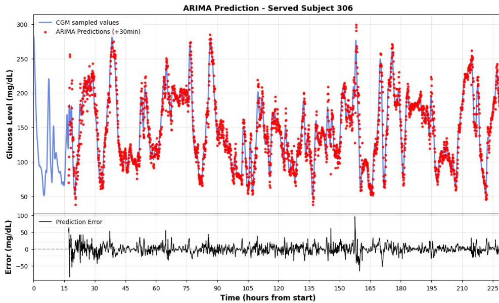
Figure 4.1 The ARIMA prediction on Hold-out set(subject 2 and 306).
