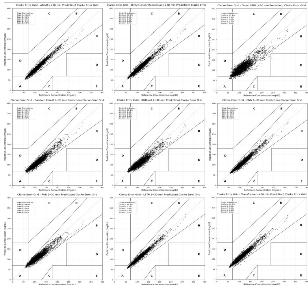
Figure 4.10 The CEG Clarke error grid of different models.
